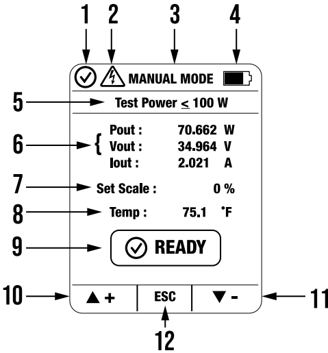
Figure 5.9 Manual mode screen. Each numbered item in the figure is defined below.
