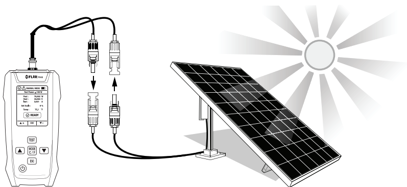
Figure 5.8 Connecting to solar panels and testing in manual mode.
