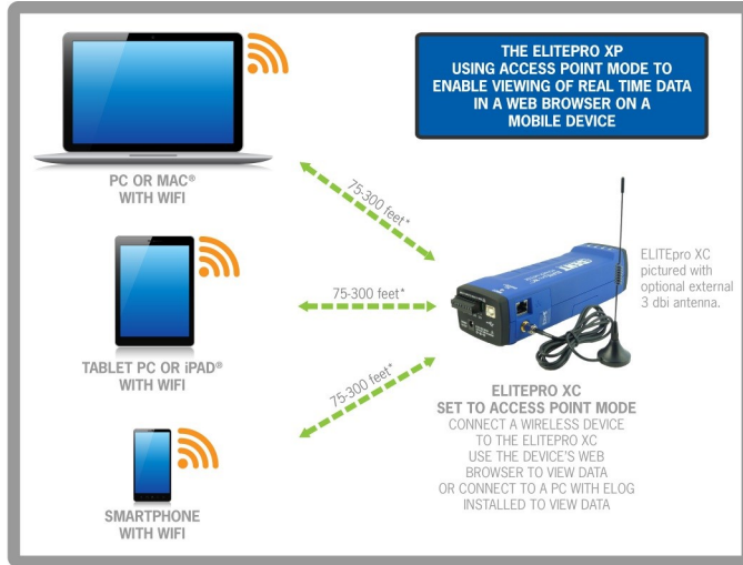
Access Point Mode using a web browser to interface with an ELITEpro XC with Wi-Fi.
