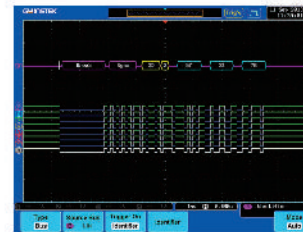
LIN Bus Trigger and Decoding Function
